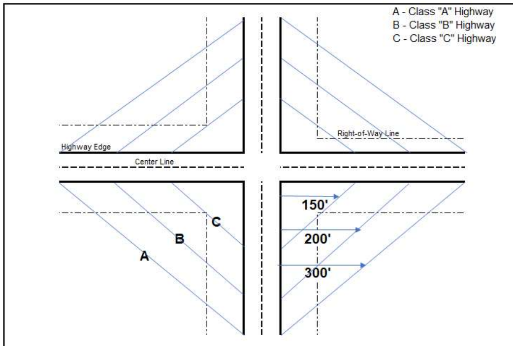
FIGURE 1: CLEAR SIGHT TRIANGLES
